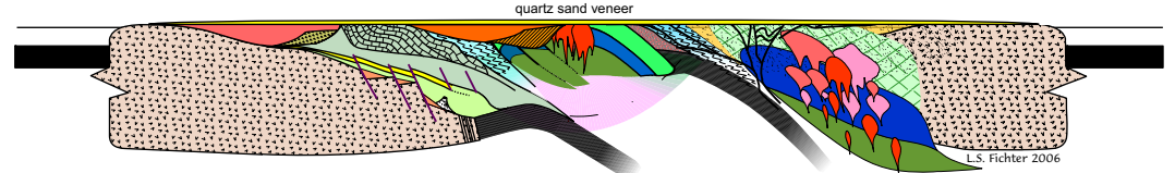
Stage I - Peneplained Continent
