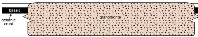
Stage C - Early Ocean Basin Formation
