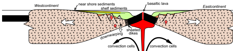
Stage D - Full Ocean Basin
