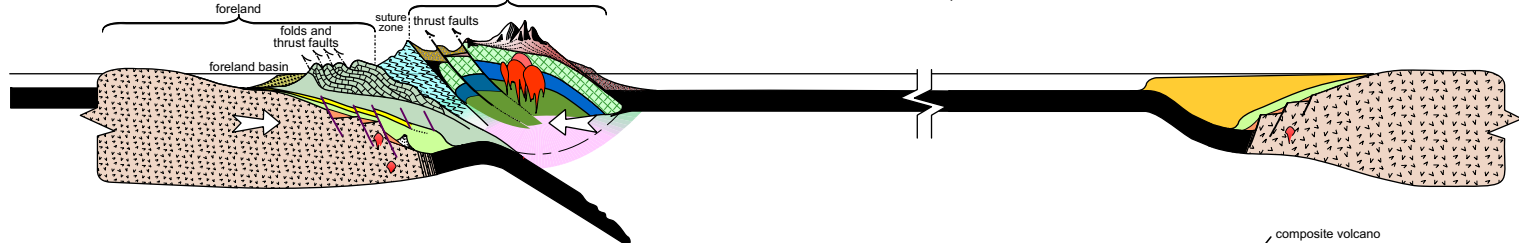
Stage G - Cordillera Mountain Building
