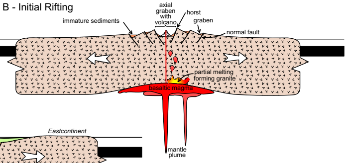
Stage B - Initial Rifting
