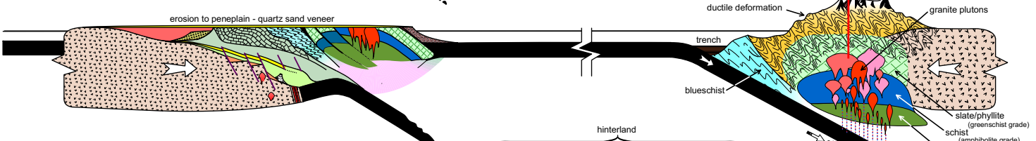
Stage H - Continent-Continent Collision
